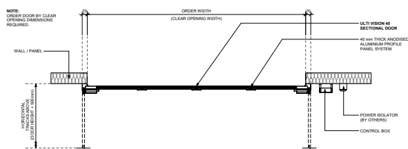
FLOOR PLAN VIEW
