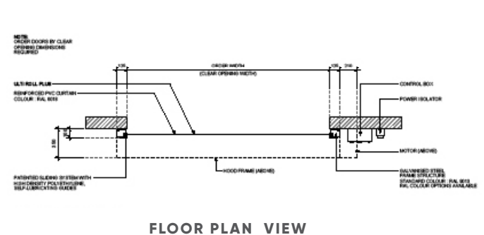
FLOOR PLAN VIEW
