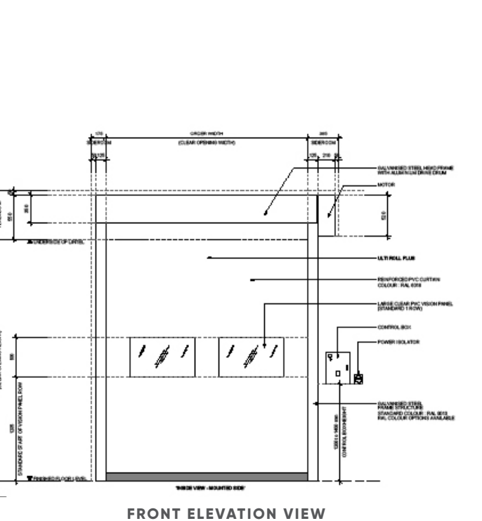
FRONT ELEVATION VIEW
