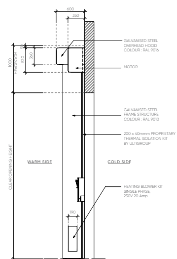
SIDE ELEVATION VIEW
