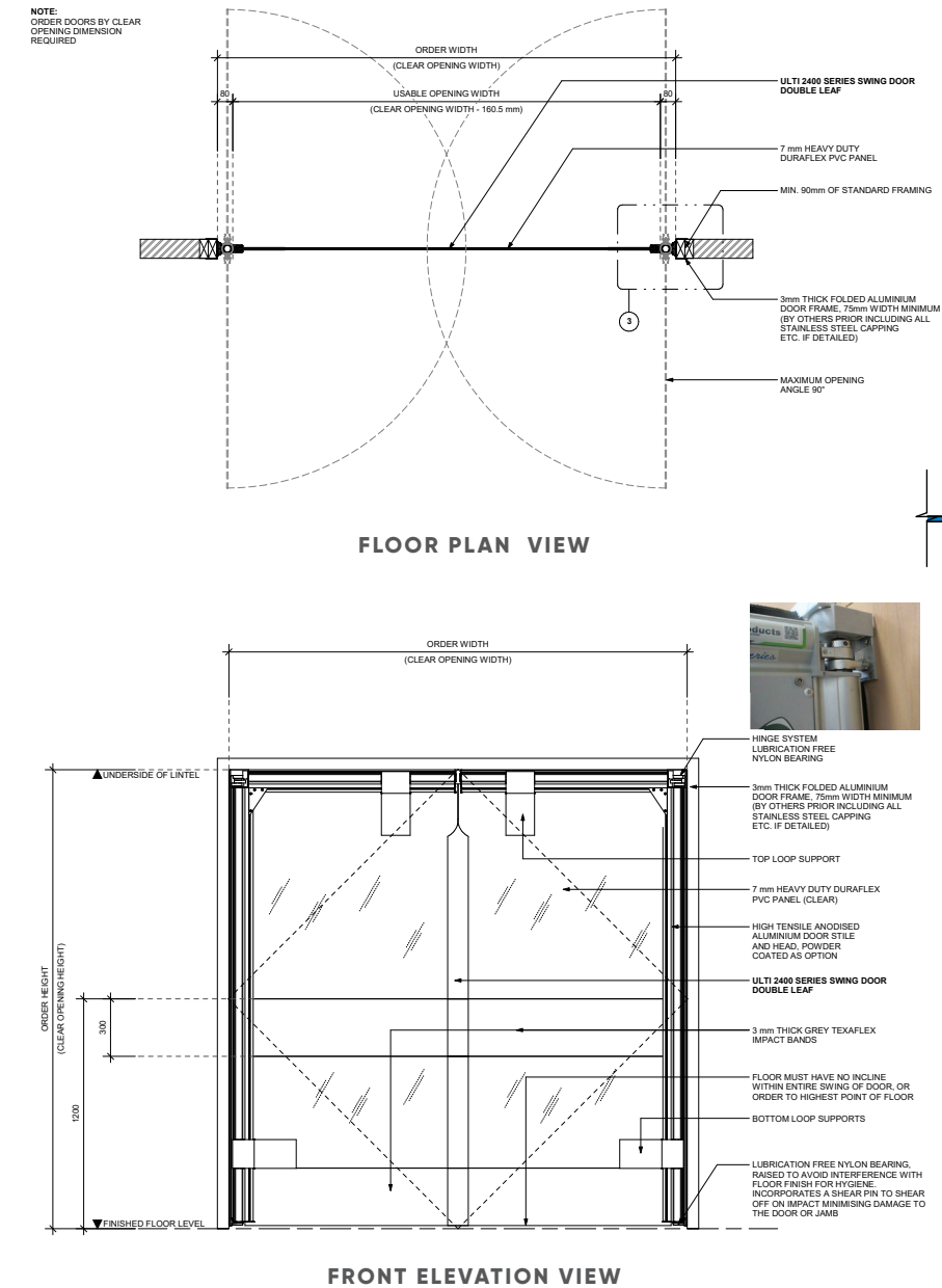
ULTI TYPICAL HINGED DOOR FRAME PREPARATION
