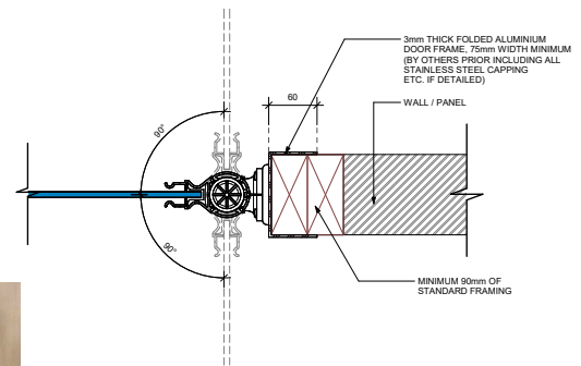
ULTI TYPICAL HINGED DOOR FRAME PREPARATION
