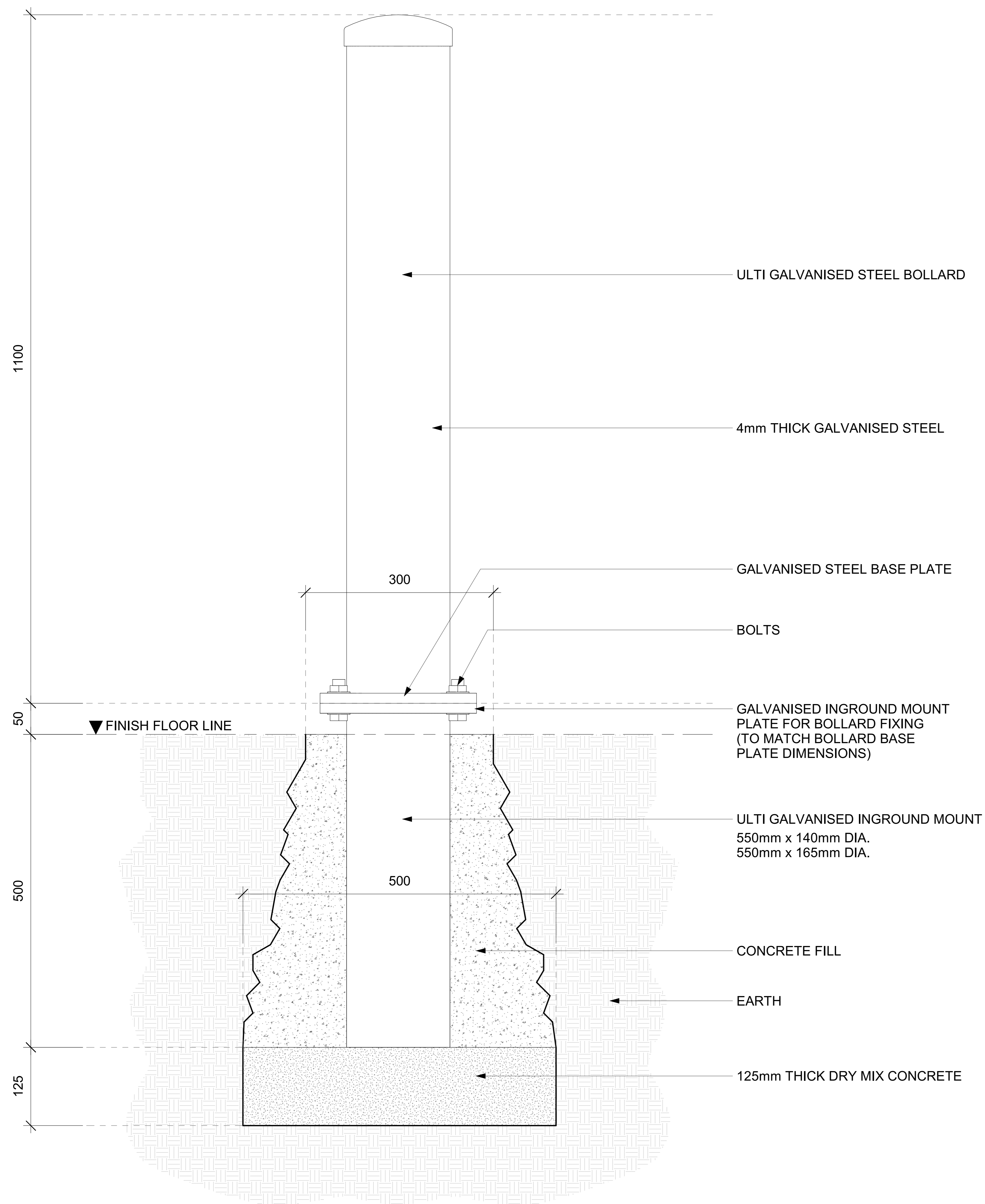
1 ELEVATION DETAIL VIEW SCALE: 1:3 MTS.
