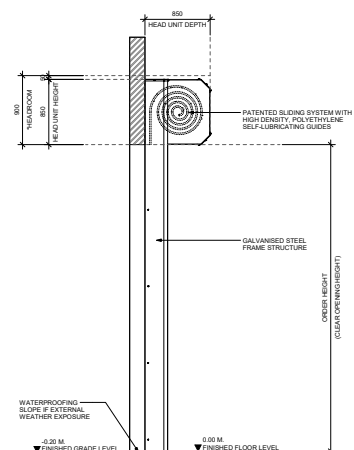
SIDE ELEVATION VIEW
