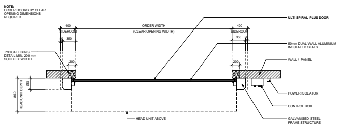
FLOOR PLAN VIEW
